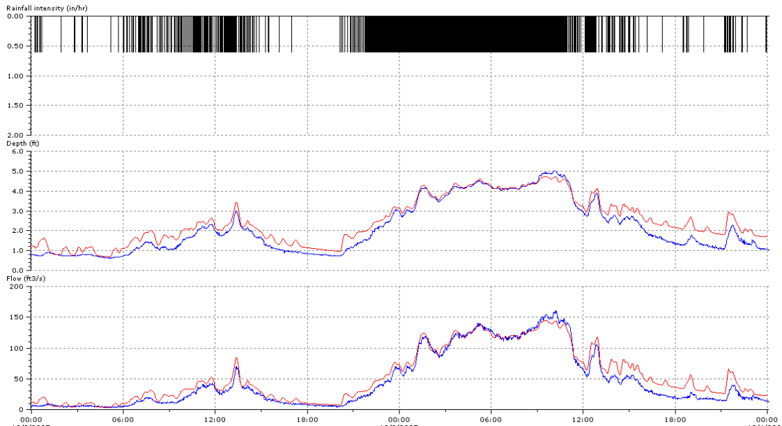
Figure 7-7 Example of Calibration Comparing Simulated and Observed Flow
