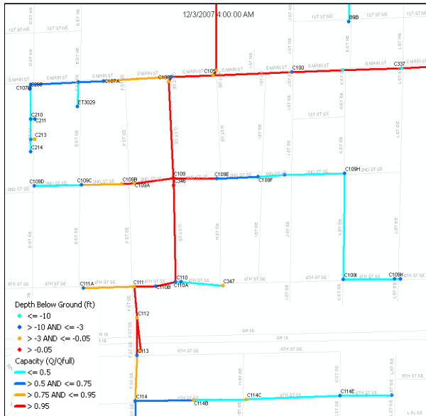
Figure 7-9 Plan View: Capacity Assessment Simulation Results
