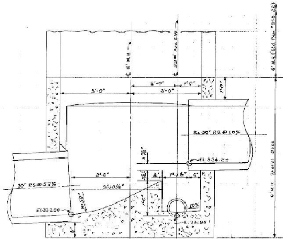
Figure 7-1 Example of Leaping Weir
