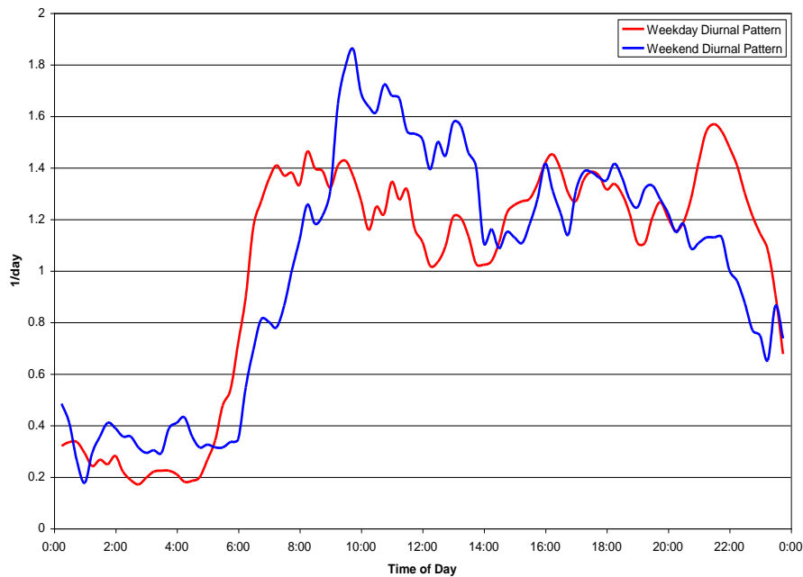
Figure 7-3 Example of Base Sanitary Flow Diurnal Patterns
