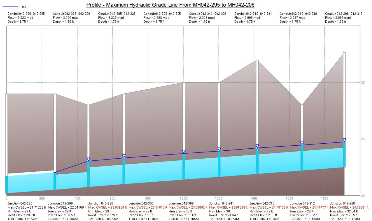
Figure 7-10 Profile View: Capacity Assessment Simulation
