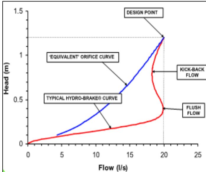
Figure 7-2 Head vs. Flow Performance Curve for a Hydrobrake
